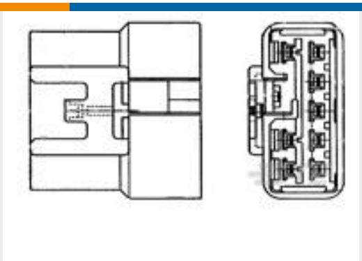
TE 产品编号175978-1 CAP HOUSING 187 (4.8 MM) ASSEMBLY
