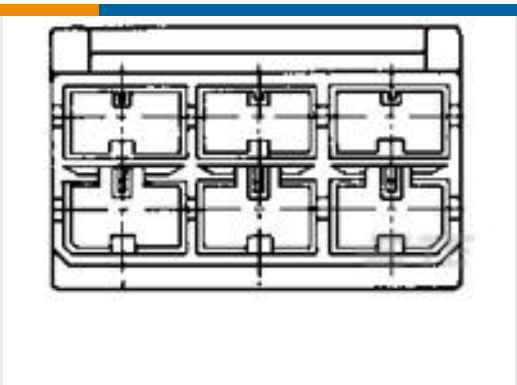
TE 产品编号926330-8 6P POS-LOCK BU GEH
