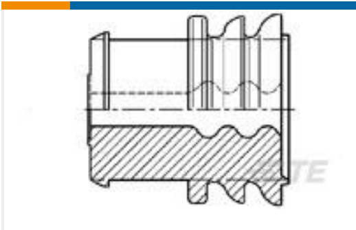
TE 产品编号100132-1 CAVITY PLUG
