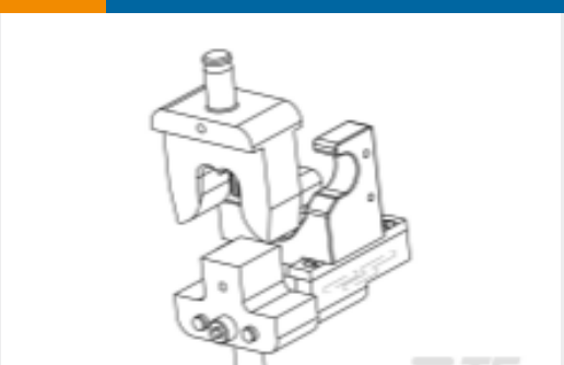
TE 产品编号2-2266559-1 OCEAN_2.0_APPLICATOR-S-055F116O
