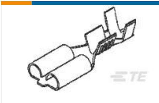
TE 产品编号170384-1 250 FASTON, REC., 22-20 AWG, BR
