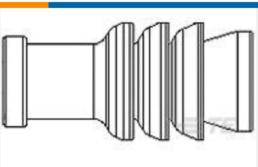
TE 产品编号963142-1 MQS SINGLE-WIRE SEAL FOR 4MM
