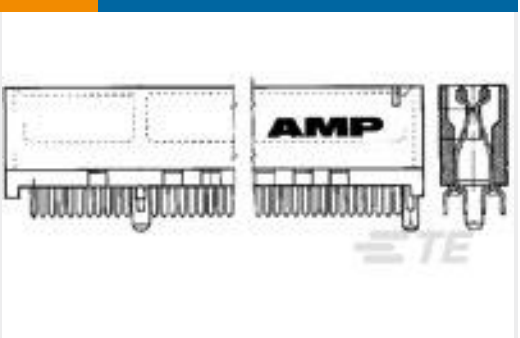
TE 产品编号1-5650090-2 STANDARD EDGE .050 SERIES 30 DUAL ASSY
