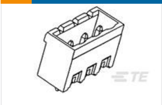
TE 产品编号1-796636-0 10POS 5.08MM CE VRT HDR,TRM BK
