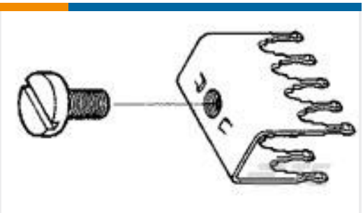
TE 产品编号1-5055323-0 10 POWER TAP ASSY .125
