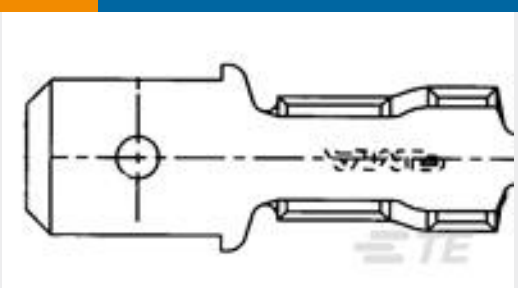
TE 产品编号180353-2 250 FASTON,TAB,12-10 AWG,TPBR
