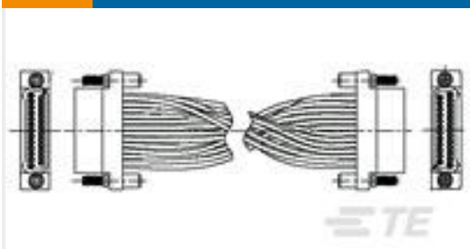
TE 产品编号766488-1 CABLE ASSY, AMPPOWER WAVE CRIMP
