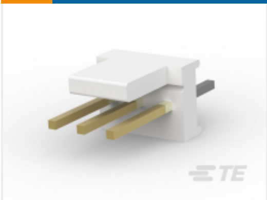
TE 产品编号1-640454-1 Polyester Vertical PCB Header: 2.54 mm, With Mating Alignment, Unshrouded
