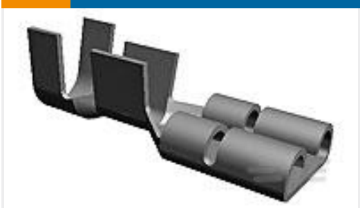
TE 产品编号1217917-2 250 FASTON, LIF REC., 18-14 AWG, BR
