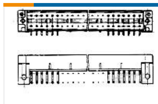
TE 产品编号172457-1 POST HDR ASSY 24P MULTI TAP
