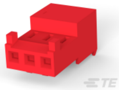
TE 产品编号5-643814-8 Nylon Tin Plated Receptacle: 2.54mm, With Mating Alignment, MTA 100
