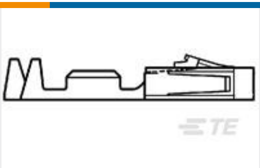
TE 产品编号104479-9 SHORT POINT CONT 15 DPLX STMPD LF
