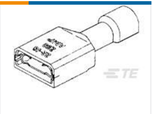
TE 产品编号2-520932-2 ULTRA-FAST .110/.125 ASY REC 22-18 TPBR
