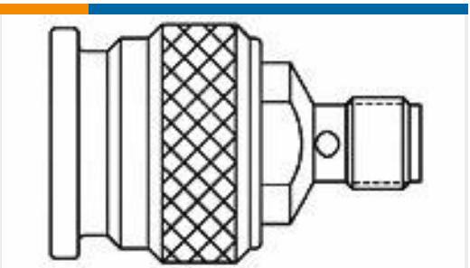
TE 产品编号1057853-1 3182 2240 00,TNC PLUG TO OSM
