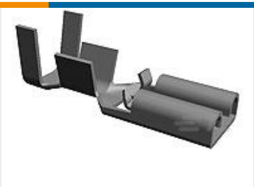
TE 产品编号1217097-2 PL 187 TERMINAL REC 22-18 AWG TPBR
