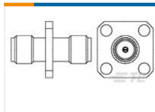
TE 产品编号1054988-1 SMA Jack-Jack Adapter 2084 8002 92
