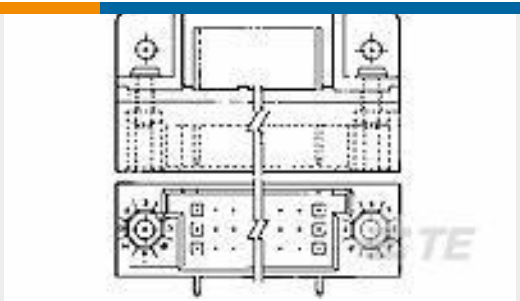
TE 产品编号533288-2 HDI PIN ASSY 3 ROW 90 POS R/A
