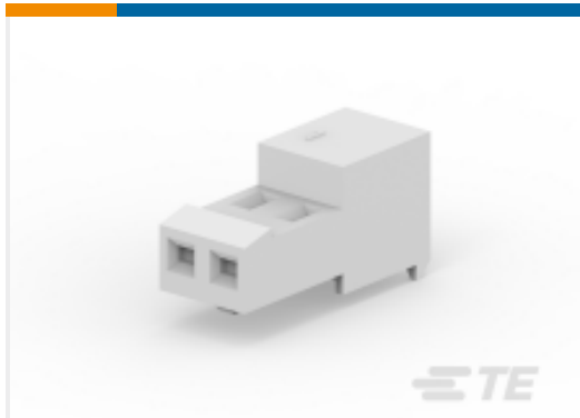
TE 产品编号3-644426-7 Nylon Tin Plated Receptacle: 2.54mm, No Mating Alignment, MTA 100
