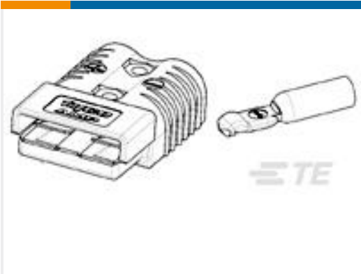
TE 产品编号1604042-6 KIT,175A,1/0 AWG,BLACK
