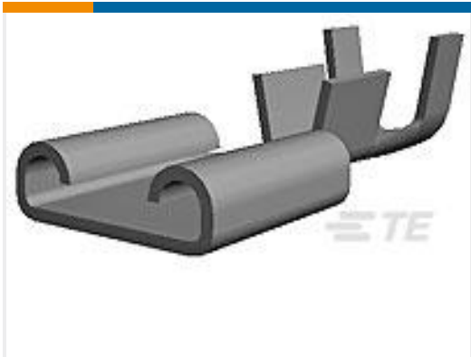
TE 产品编号62998-2 FASTON 250 RECEPTACLE 10-8 AWG TPBR
