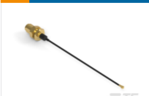
TE 产品编号2016695-2 RF CA,RP-SMA BULKHEAD TO UMCC IV,L100MM
