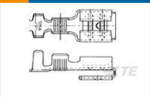
TE 产品编号160739-2 250 FASTON, PIGGYBACK REC., 18-14 AWG, TPBR
