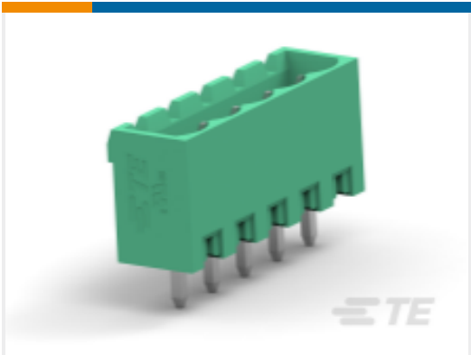
TE 产品编号2351885-2 2POS TB HDR 180 DEG, PITCH 5.0&TL 4.5mm
