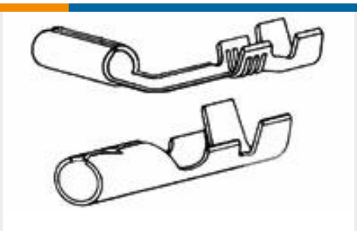
TE 产品编号42142-2 SHUR PLUG TERMINAL 18-14 AWG BR
