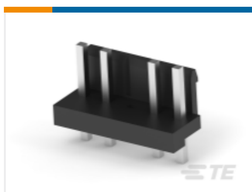
TE 产品编号8-1717011-4 EP CONN.HDR ASSY 4/5P BLACK (NO.3 POST)
