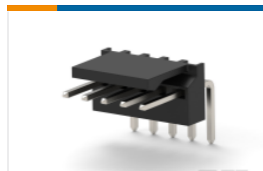
TE 产品编号3-647051-2 Nylon Right Angle PCB Header: 2.54 mm, Wire-to-Board, Through Hole, MTA 100
