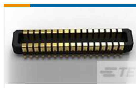
TE 产品编号2-2201196-4 0.4 STACKING CONN H0.98 PLUG ASSEMBLY
