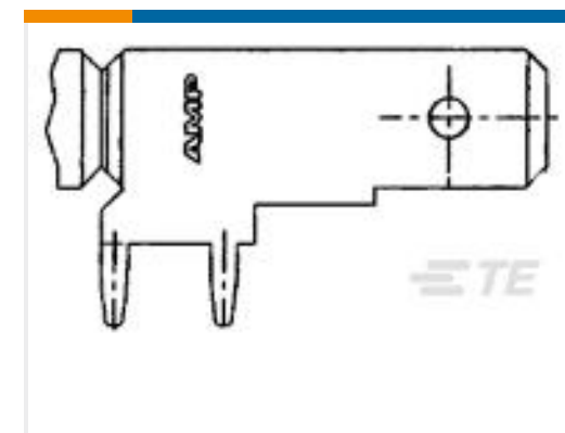
TE 产品编号1217754-1 250 FASTON, FLAG, PCB TAB, TNBR
