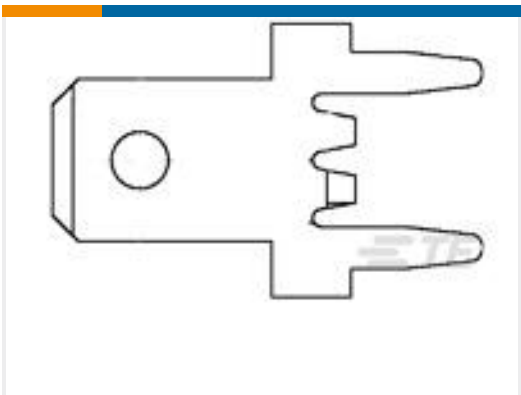
TE 产品编号1217133-1 187 FASTON,PCB TAB,TNBR
