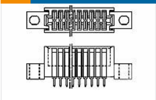
TE 产品编号1-166089-5 DUAL LOADED/WITH EARS
