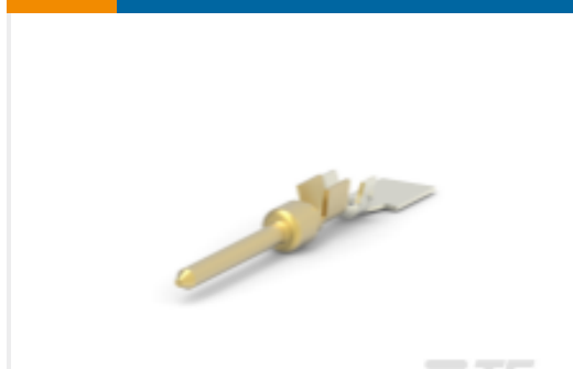
TE 产品编号166995-2 D-Sub Connector Contacts: Pin, Brass, Signal, Size 20
