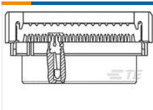
TE 产品编号2-111626-7 026 2MM 30DP FT
