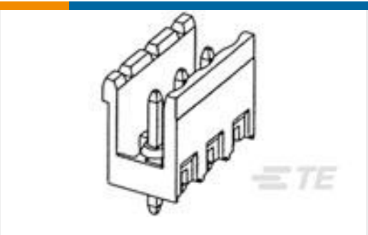
TE 产品编号282825-6 TERMI-BLOK HEADER,ASSY90 6P.5,
