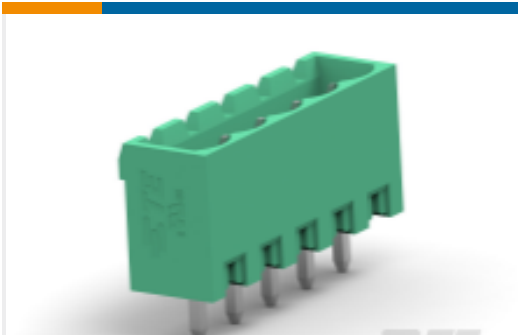
TE 产品编号2351885-2 2POS TB HDR 180 DEG, PITCH 5.0&TL 4.5mm
