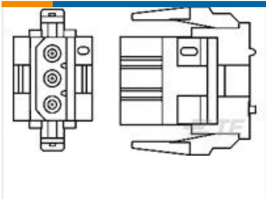
TE 产品编号1-640518-0 03P MR II PLUG HSG V0 RED
