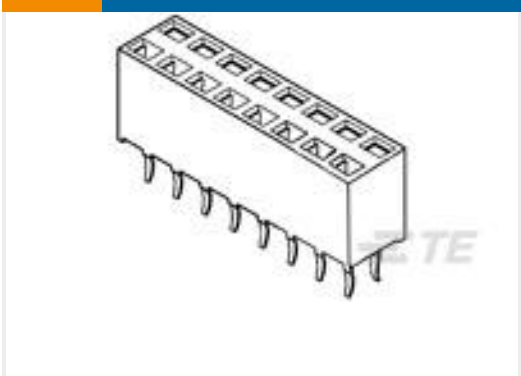
TE 产品编号1-215307-0 2X10P HV100 REC CON. TE, 7.0MM
