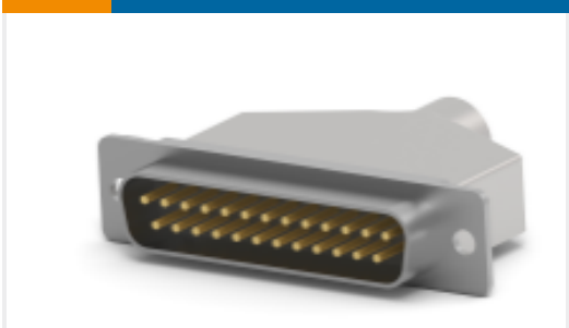
TE 产品编号1-747950-5 IDC D-Sub: Connector Kit, Plug, Wire to Wire, Signal, 2.77 mm
