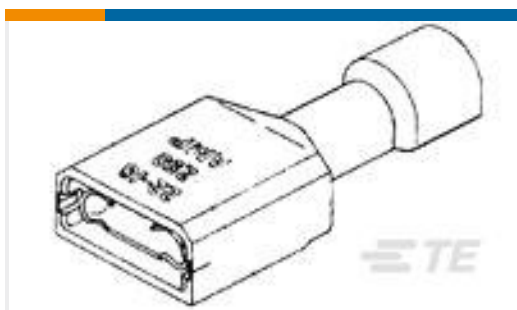
TE 产品编号2-520184-2 ULTRAFast 250 ASSY REC 22-18 TPBR LP
