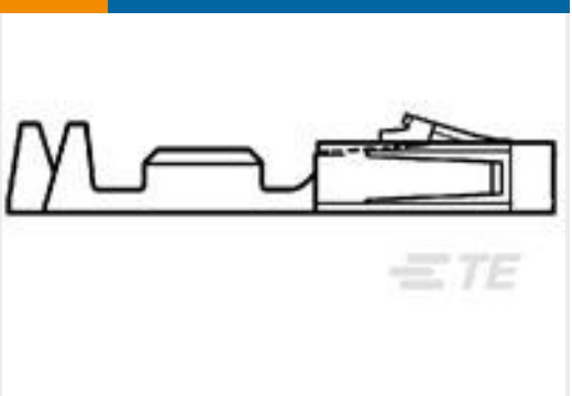
TE 产品编号104479-9 SHORT POINT CONT 15 DPLX STMPD LF
