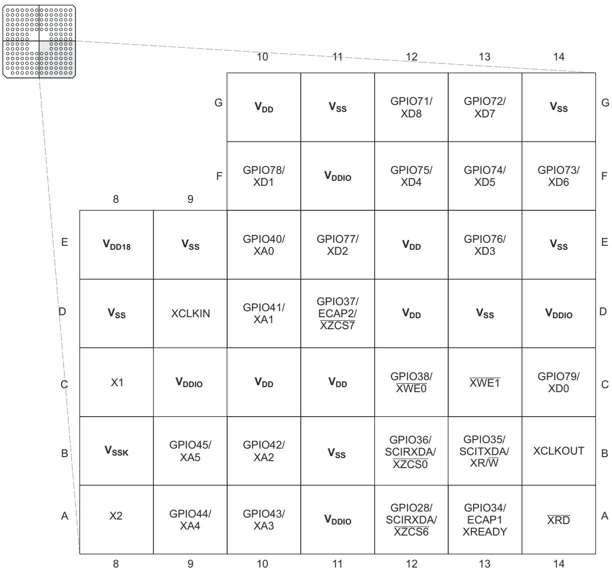
图 6-4. C2834x 179-Ball ZHH MicroStar BGA Lower-Right Quadrant (Bottom View)
