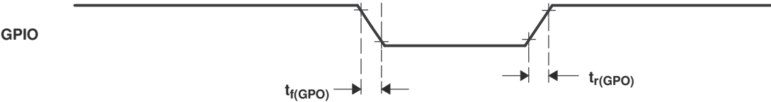
图 7-7. General-Purpose Output Timing
