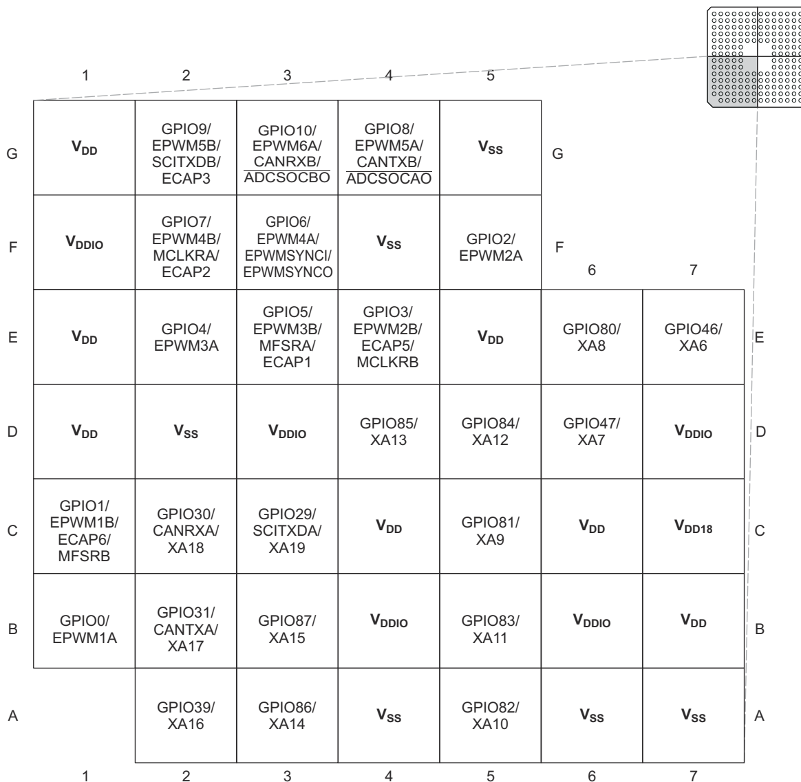
图 6-3. C2834x 179-Ball ZHH MicroStar BGA Lower-Left Quadrant (Bottom View)
