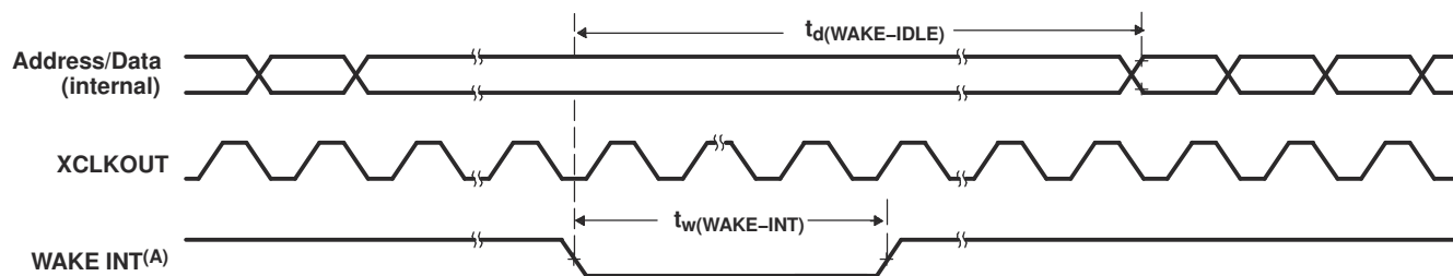
图 7-10. IDLE Entry and Exit Timing
