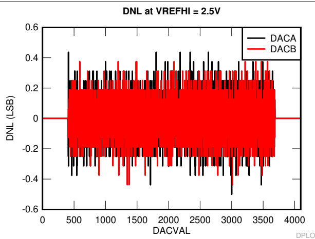
Figure 7-42. DNL
