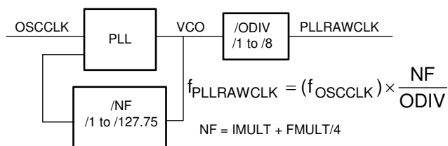
Figure 7-11. System PLL
