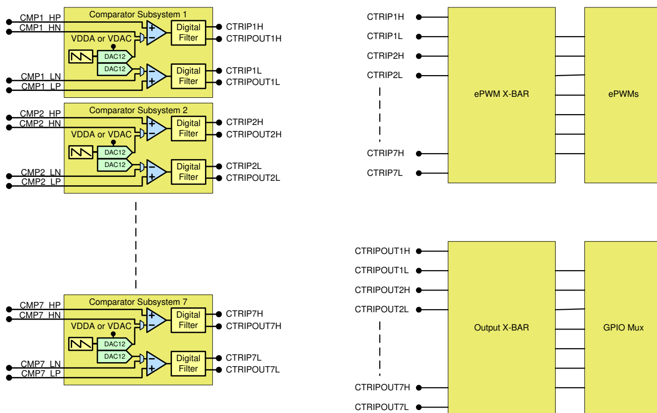
Figure 7-48. CMPSS Connectivity
