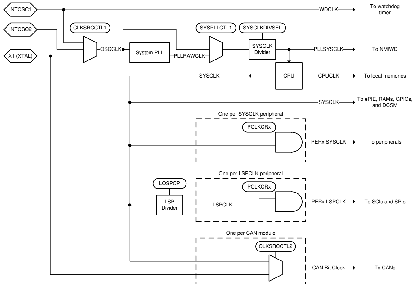
Figure 7-10. Clocking System
