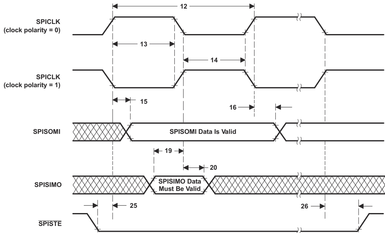
Figure 7-77. SPI Slave Mode External Timing (Clock Phase = 0)
