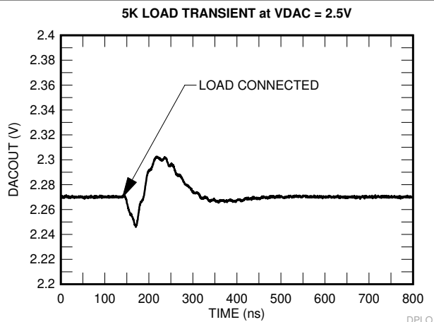
Figure 7-47. 5-k \Omega Load Transient
