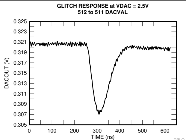
Figure 7-45. Glitch Response – 512 to 511 DACVAL
