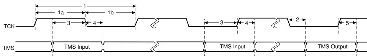
Figure 7-20. cJTAG Timing
