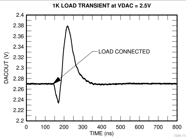
Figure 7-46. 1-k \Omega Load Transient
