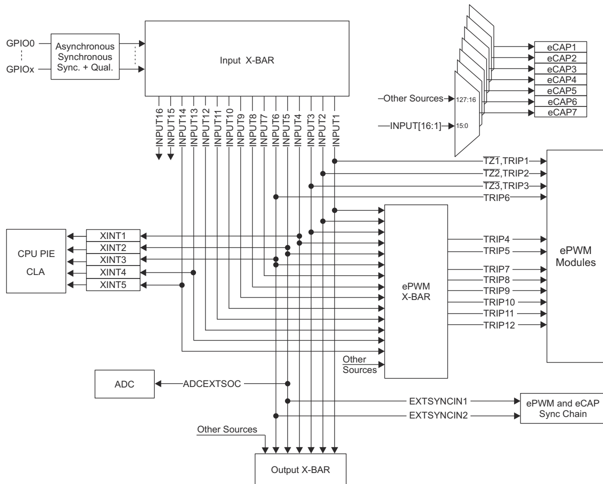
Figure 6-5. Input X-BAR
