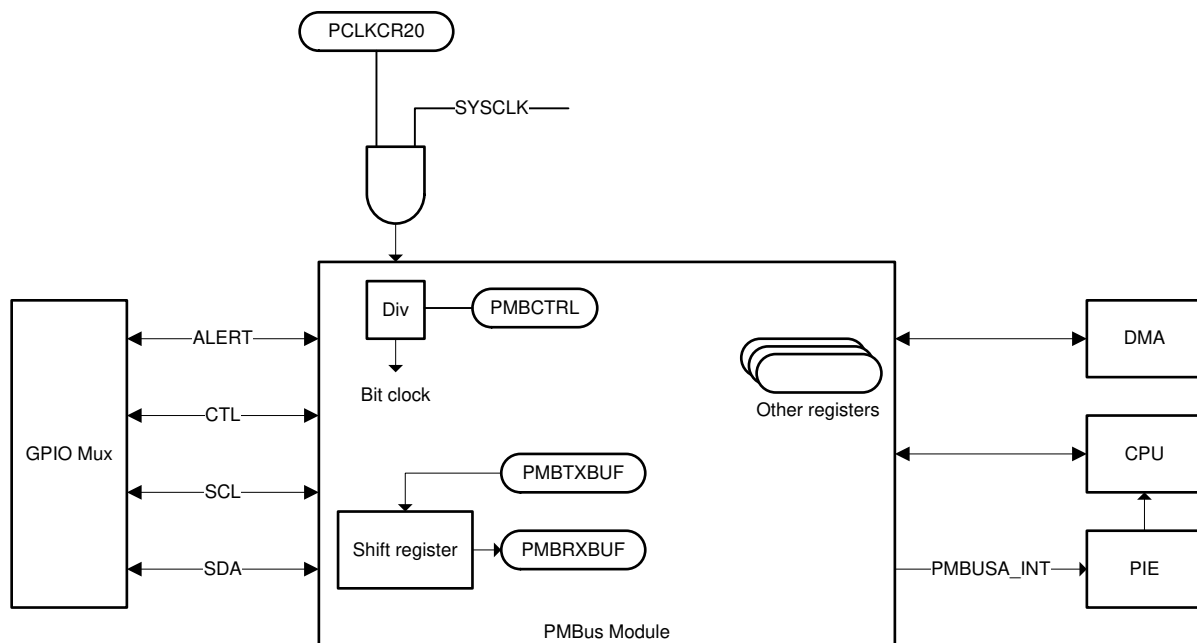
Figure 7-72. PMBus Block Diagram
