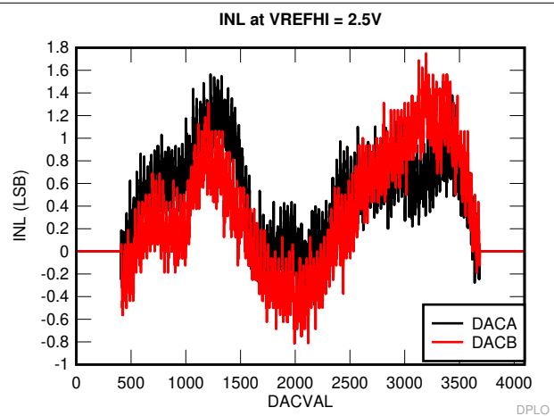
Figure 7-43. INL
