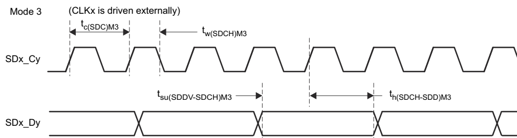
Figure 7-68. SDFM Timing Diagram – Mode 3
