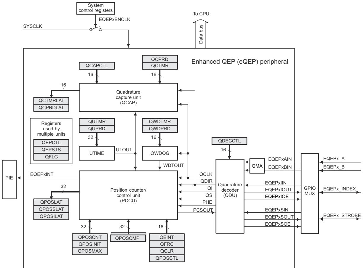
Figure 7-63. eQEP Block Diagram
