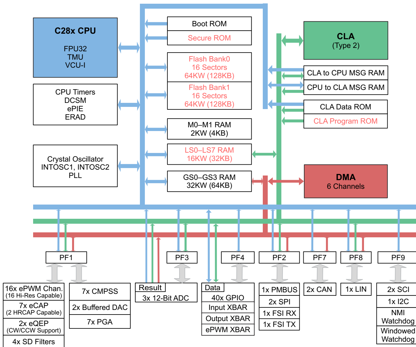
Figure 3-1. Functional Block Diagram
