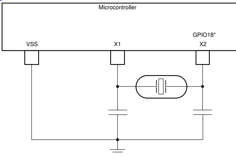
Figure 7-13. External Crystal
