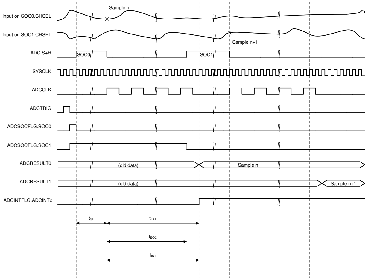
Figure 7-35. ADC Timings
