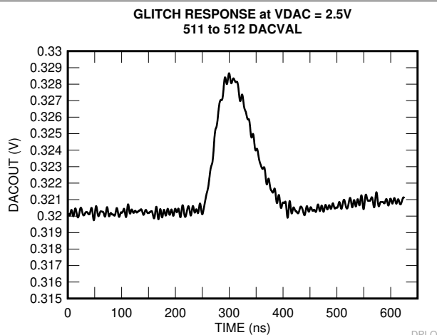
Figure 7-44. Glitch Response – 511 to 512 DACVAL
