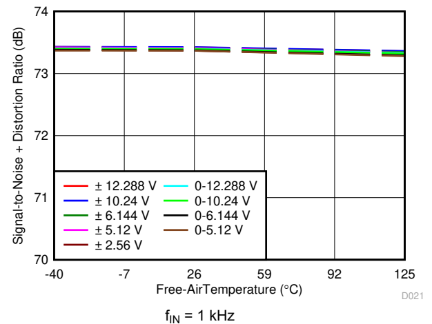
图 6-38. SINAD vs Temperature
