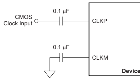
Figure 136. Single-Ended Clock Driving Circuit
