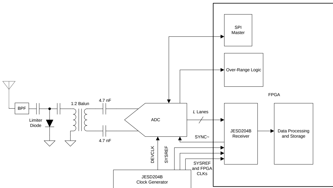
图 109. Simplified Schematic
