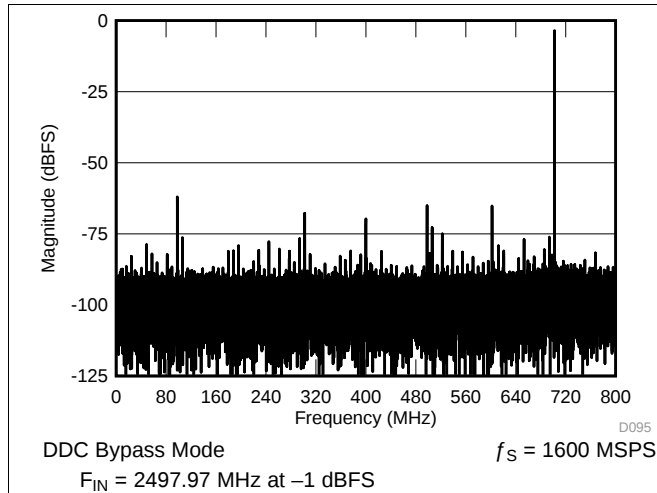
图 110. Spectrum — DDC Bypass Mode
