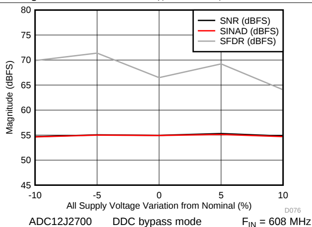
Figure 10. SNR, SINAD, SFDR vs Supply Voltage
