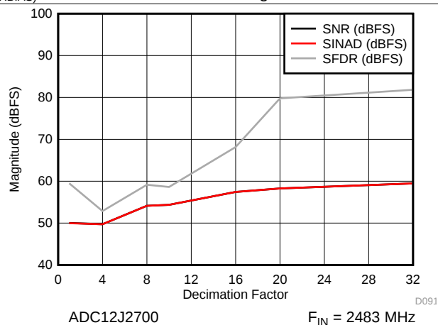
Figure 9. SNR, SINAD, SFDR vs Decimation Setting
