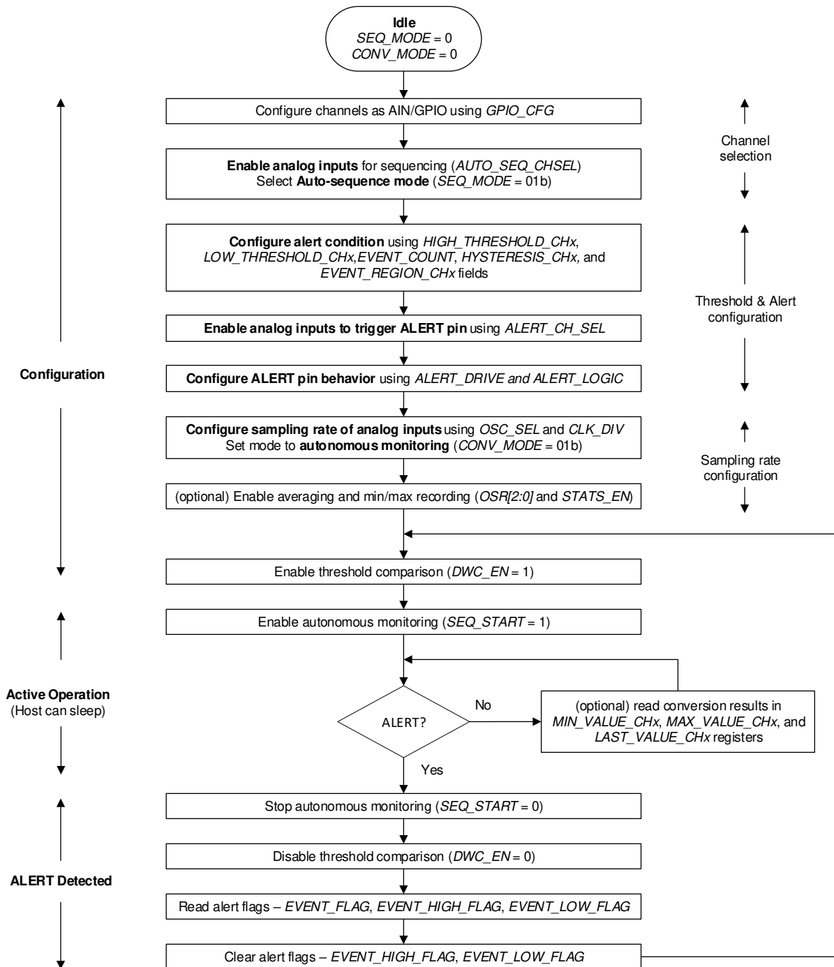
图 37. Configuring the Device in Autonomous Mode
