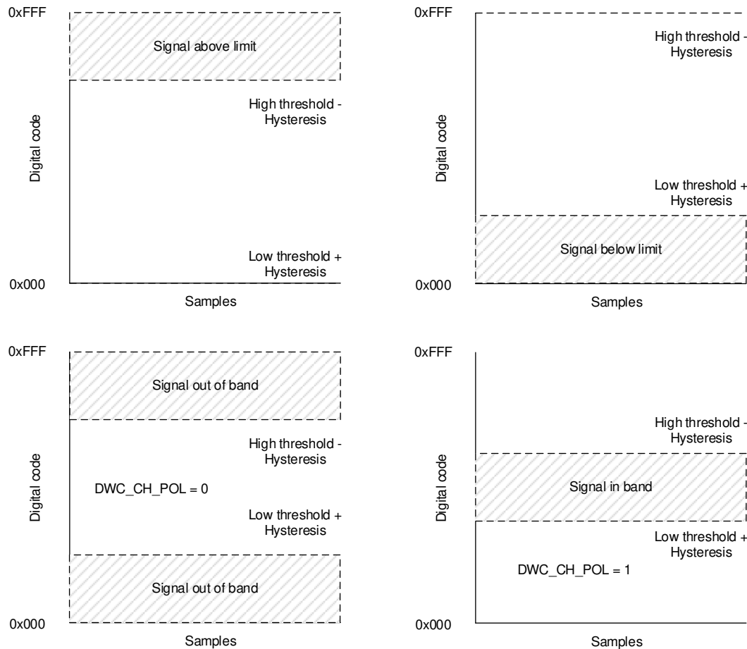
图 27. Event Monitoring With the Window Comparator
