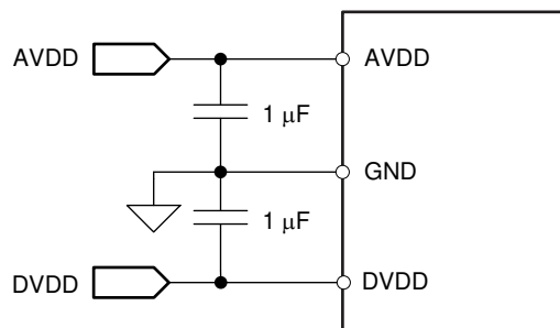
图 154. Power-Supply Decoupling
