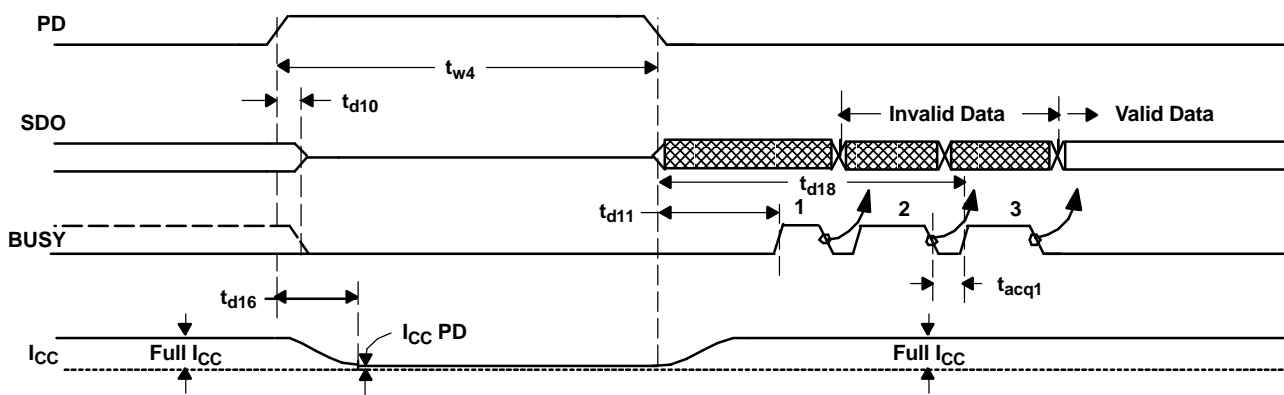
Figure 56. Device Full Power Down/Resume (External Reference Used)
