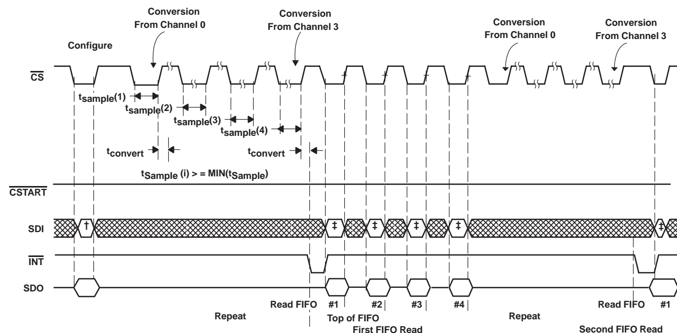
Figure 14. TLC1514/TLC1518 Mode 10/11 μp Serial Interface (conversions triggered by CS)
